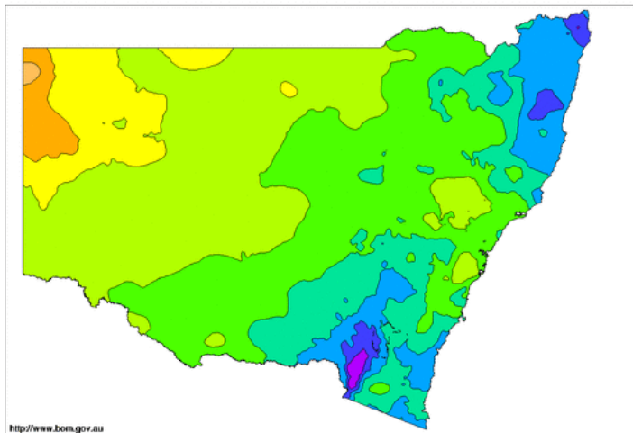
New South Wales Rainfall totals (mm) 1 August 2017 to 31 January 2018 Australian Bureau of Meteorology
