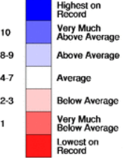
Rainfall Decile Ranges
