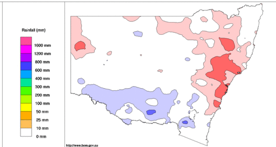
New South Wales Rainfall Deciles 1 August 2017 to 31 January 2018 Distribution Based on Gridded Data Australian Bureau of Meteorology
