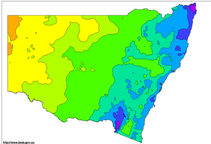
New South Wales Rainfall totals (mm) 1 February 2016 to 31 January 2018 Australian Bureau of Meteorology
