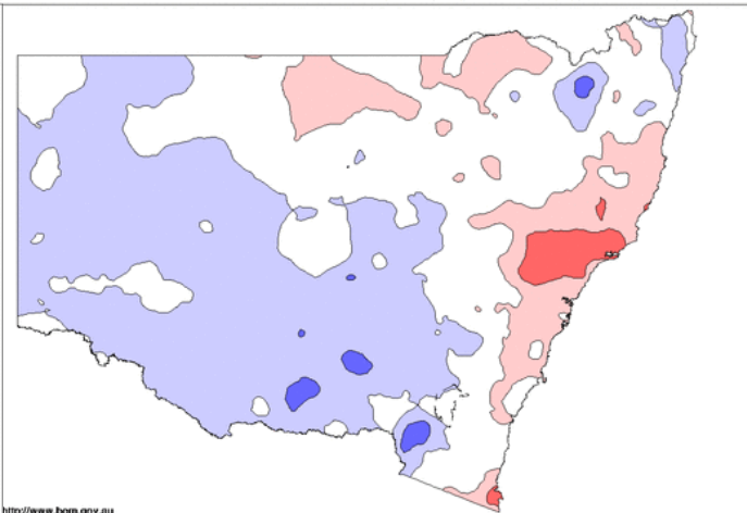
New South Wales Rainfall Deciles 1 February 2016 to 31 January 2018 Distribution Based on Gridded Data Australian Bureau of Meteorology
