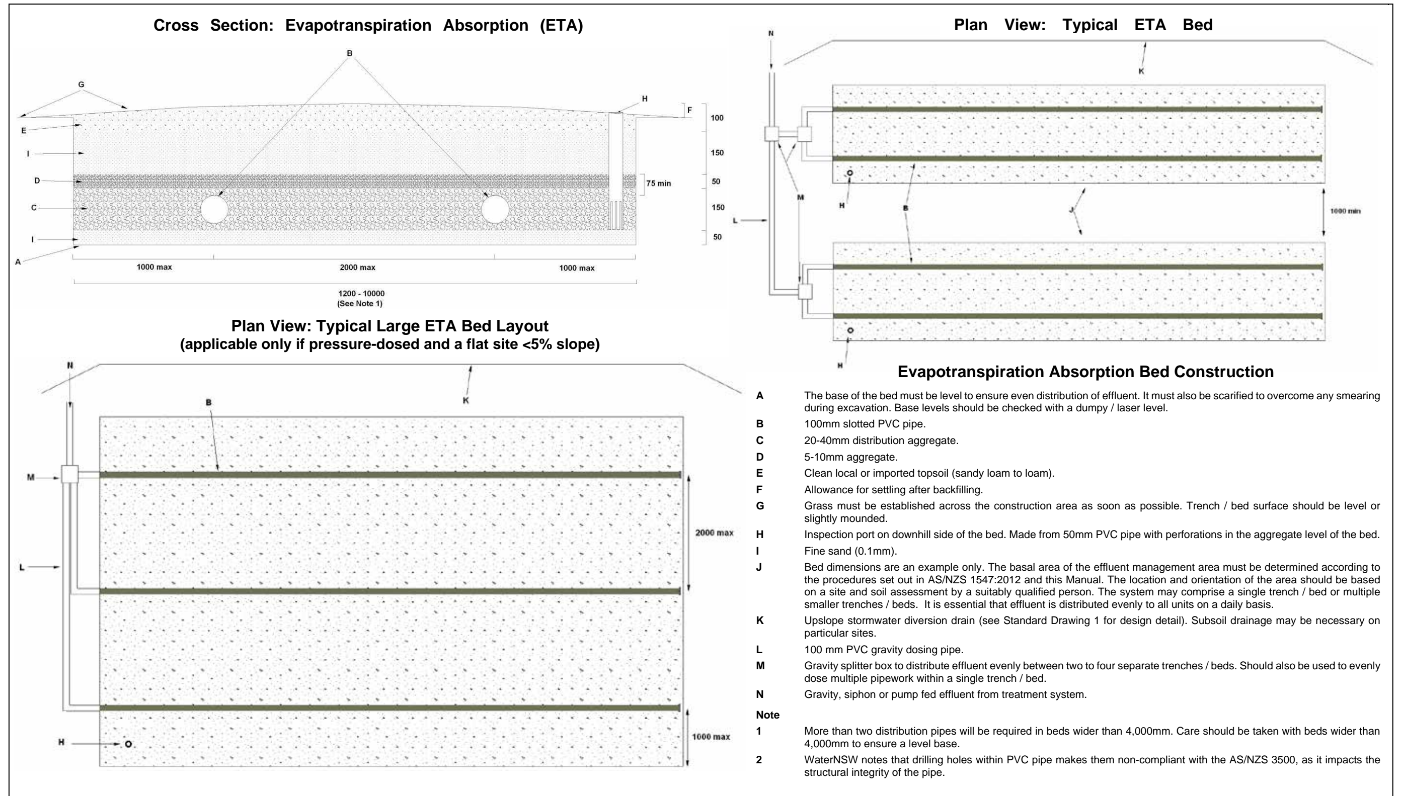
Standard Drawing 11A – Evapotranspiration Absorption Bed (not to scale)
