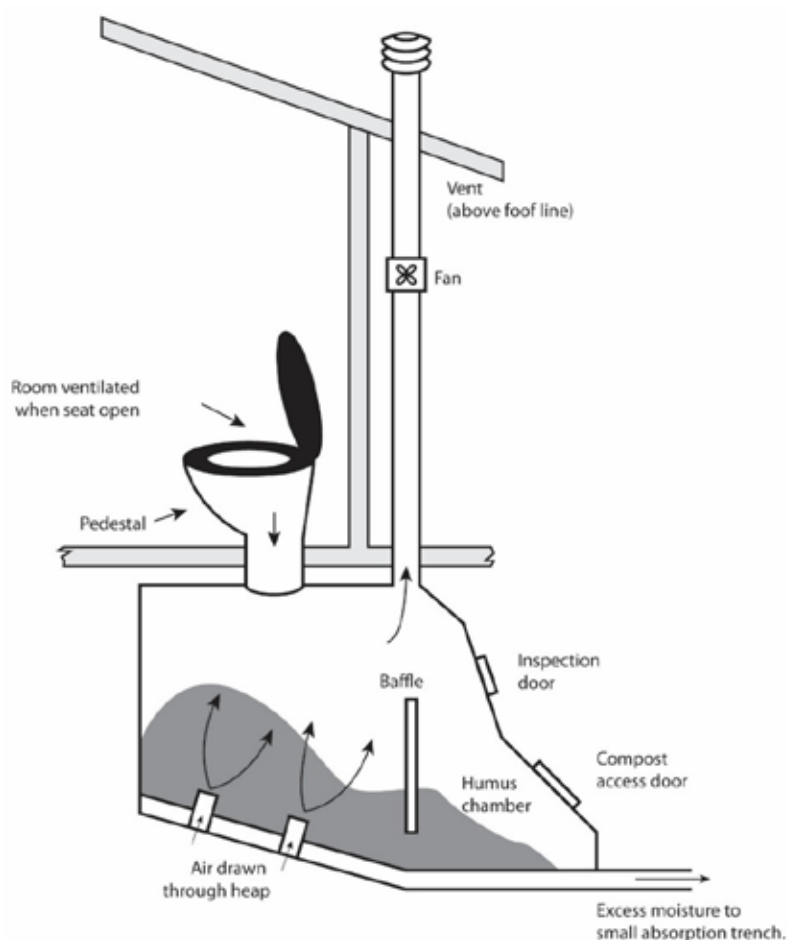
Figure 6.2 A typical section of composting toilet
