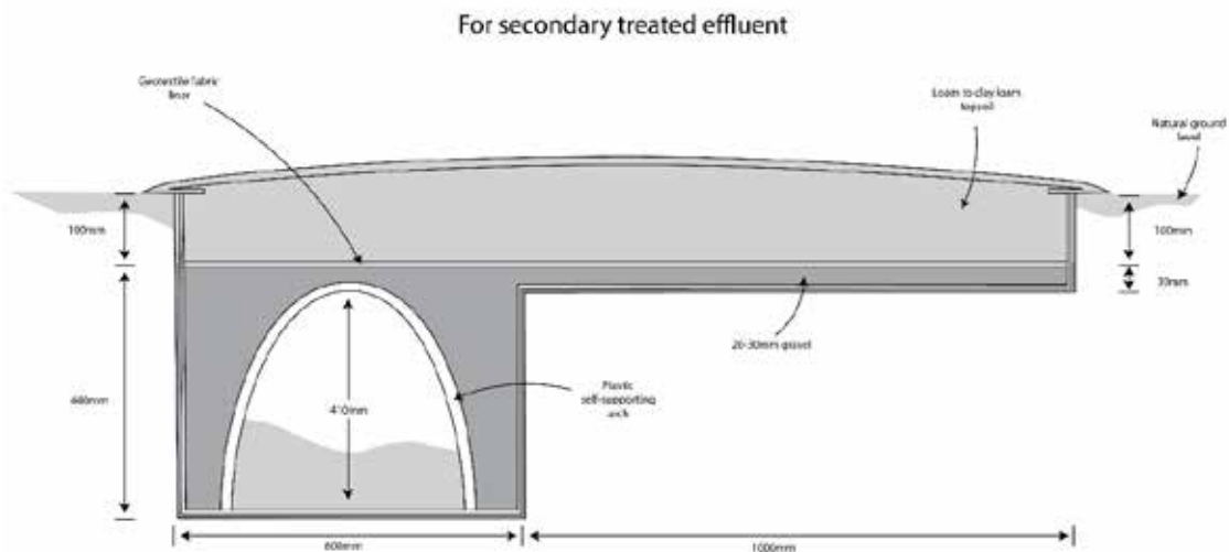
Figure 10.13b 'Wick' trench for secondary treated effluent
