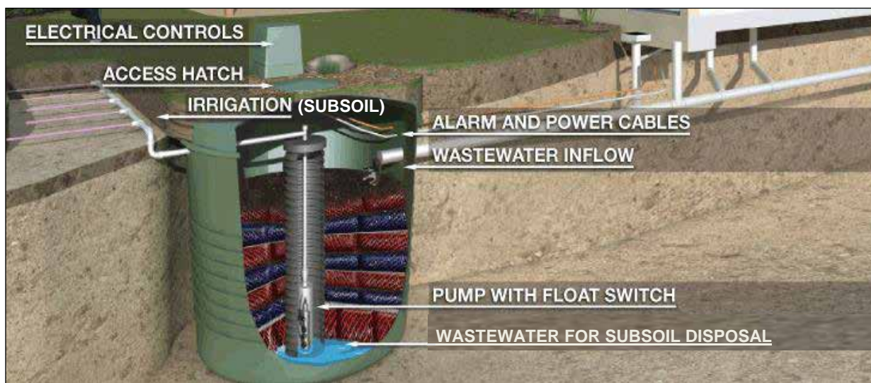
Figure 5.1 A Biological Filter System (after Biolytix, 2009)
