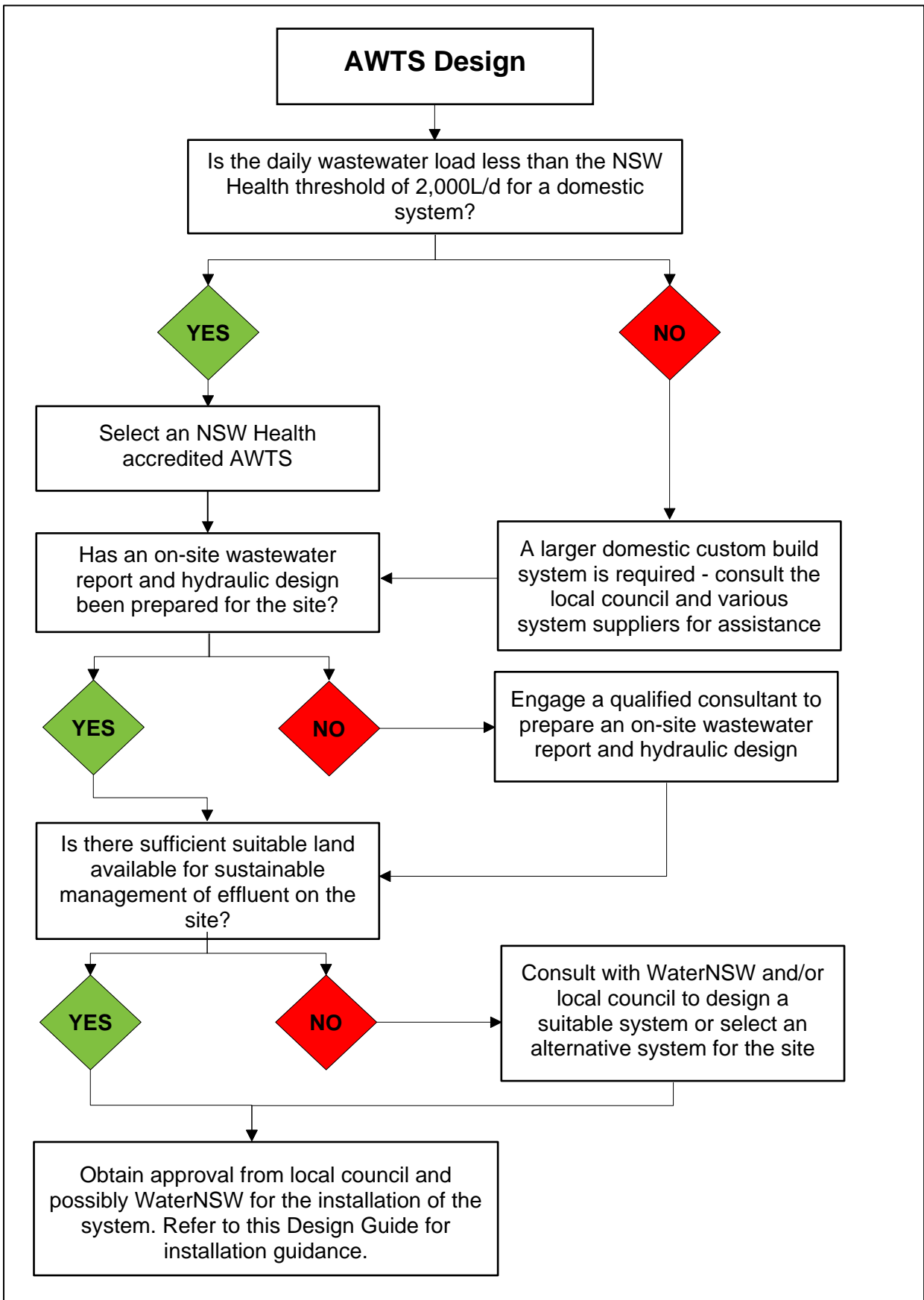
Figure 4.2 AWTS Design
