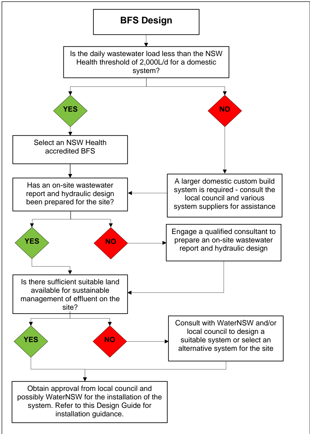
Figure 5.2 Biological filter system design
