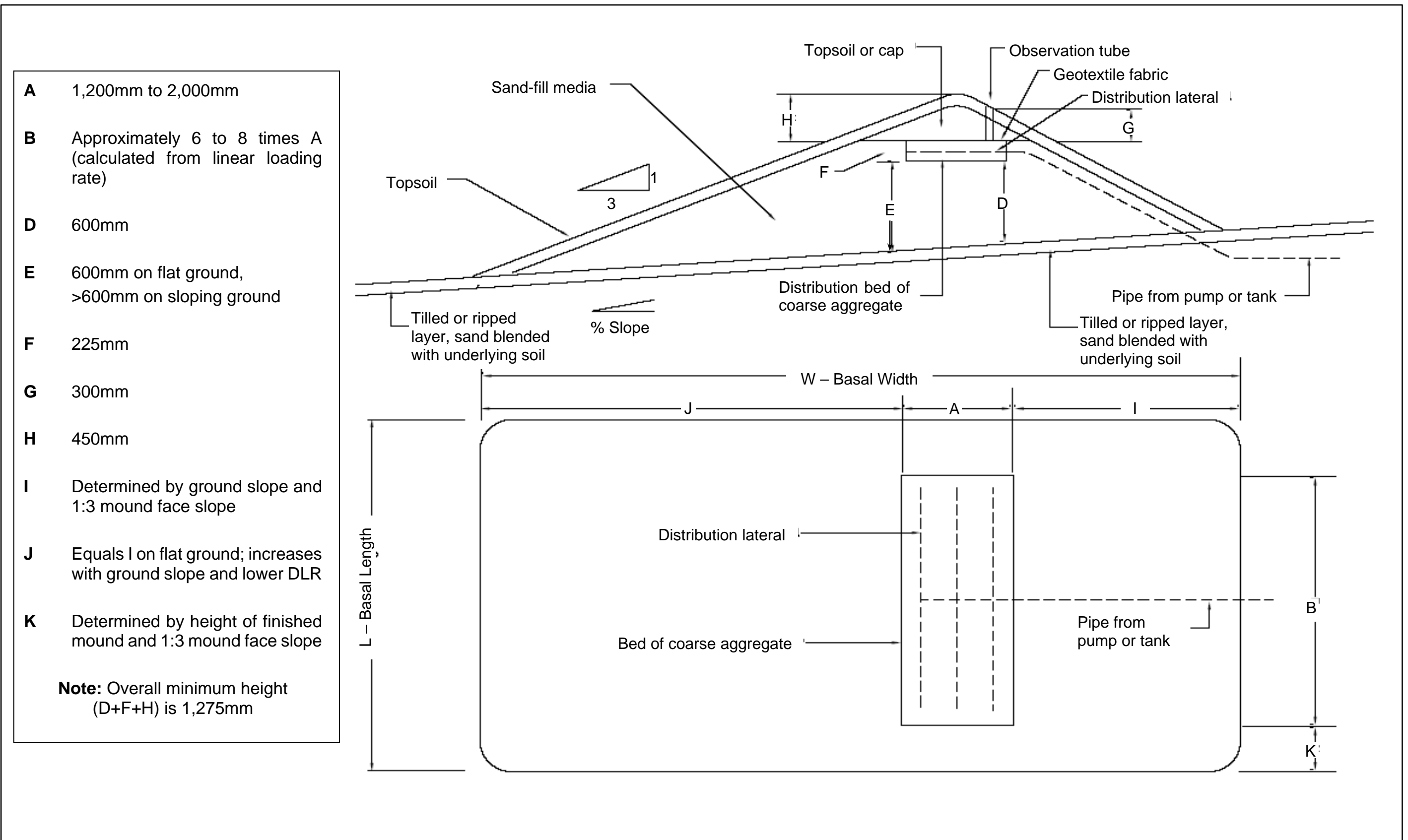
Standard Drawing 9A – Wisconsin Sand Mound (not to scale)
