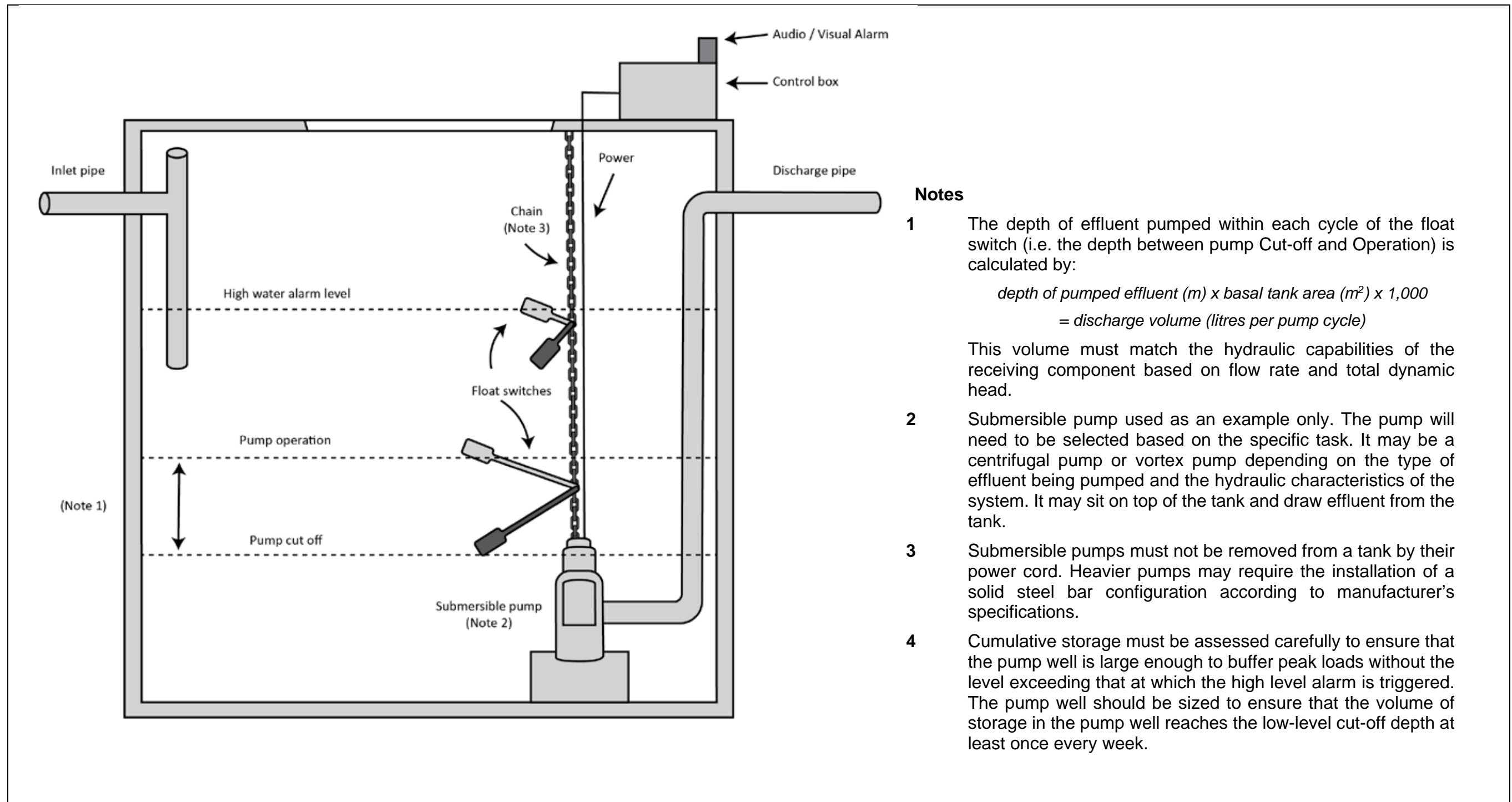
Standard Drawing 12A – Demand Dose Pump well (not to scale)
