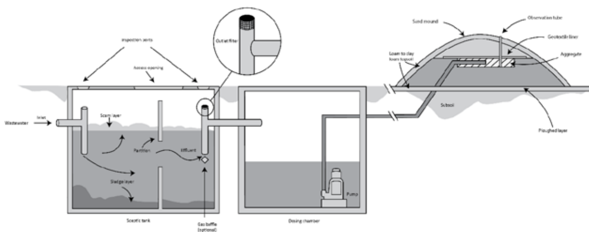
Figure 9.1 Components of a Wisconsin sand mound system
