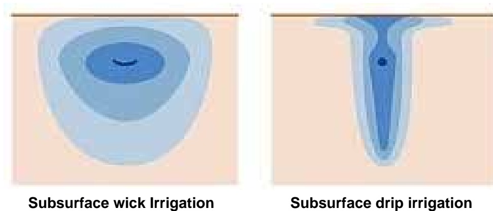
Figure 13.5 Irrigation wetting patterns
