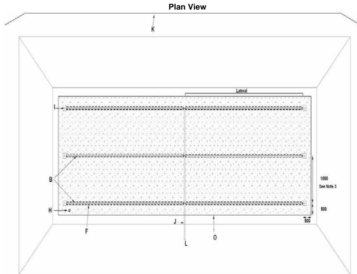
Standard Drawing 10C – Raised Pressure Dosed Absorption Bed Construction (not to scale)
