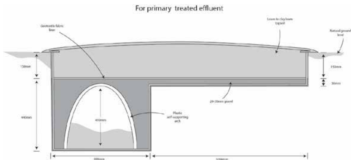
Figure 10.13a 'Wick' trench for primary treated effluent
