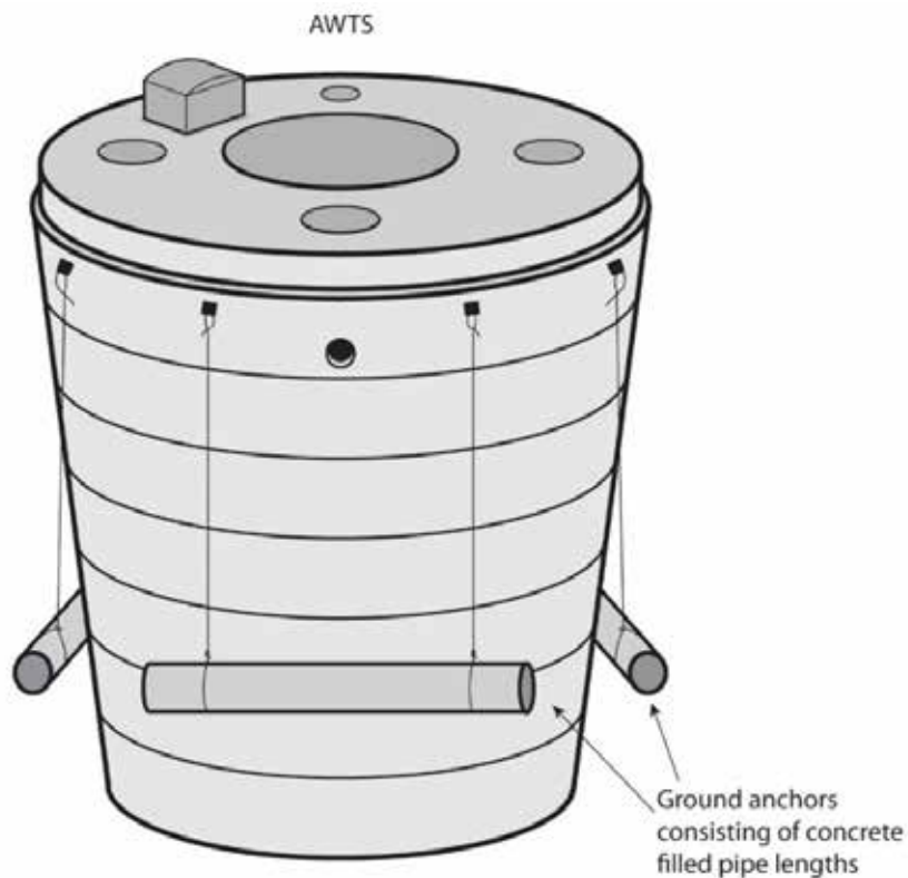
Figure 4.5 Ground anchors
