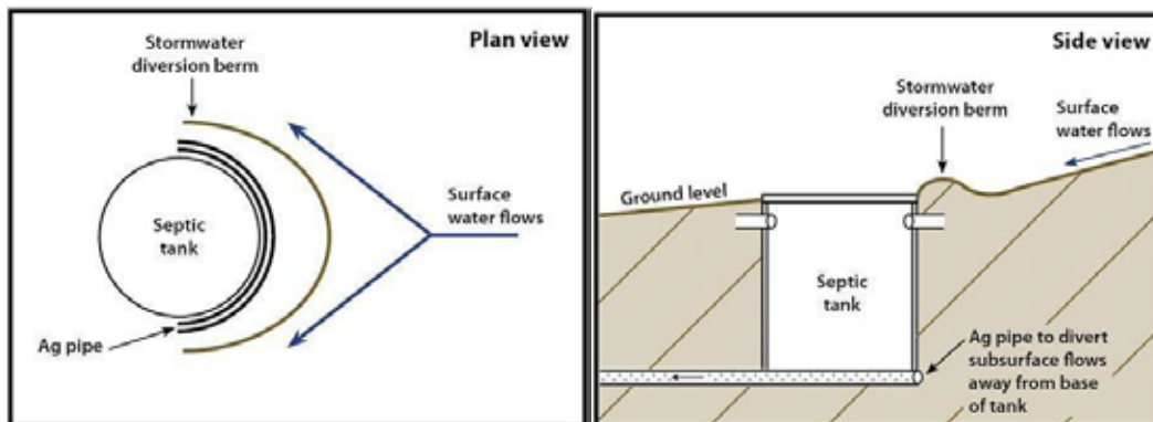
Figure 3.3 Tank stormwater drainage design
